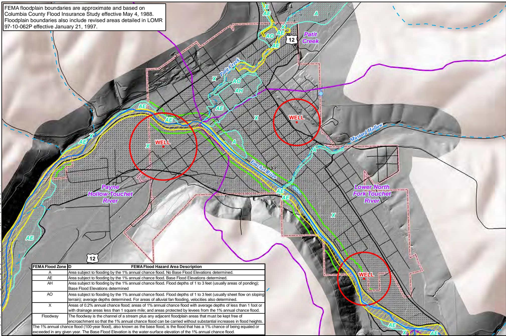
Figure 3: Topography, Floodplains, and Mapped Hydrography
